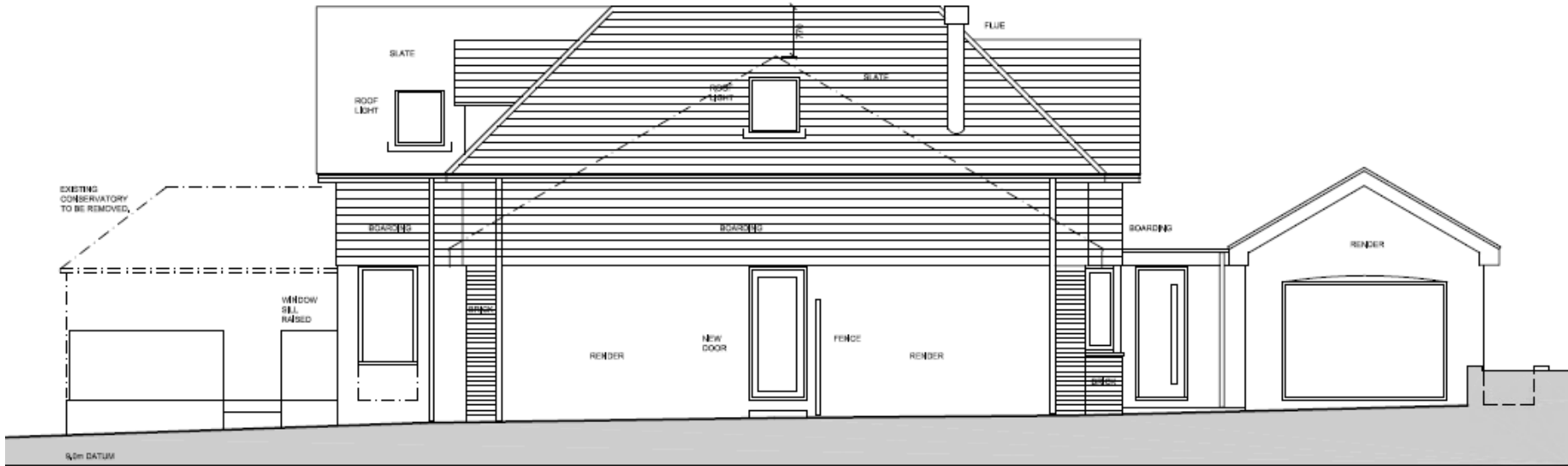
EAST ELEVATION
