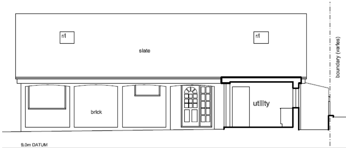
NORTH ELEVATION
