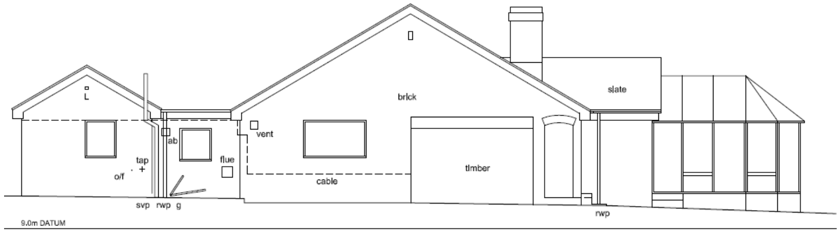
WEST ELEVATION
