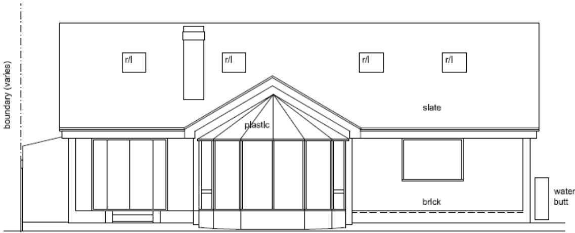
SOUTH ELEVATION
