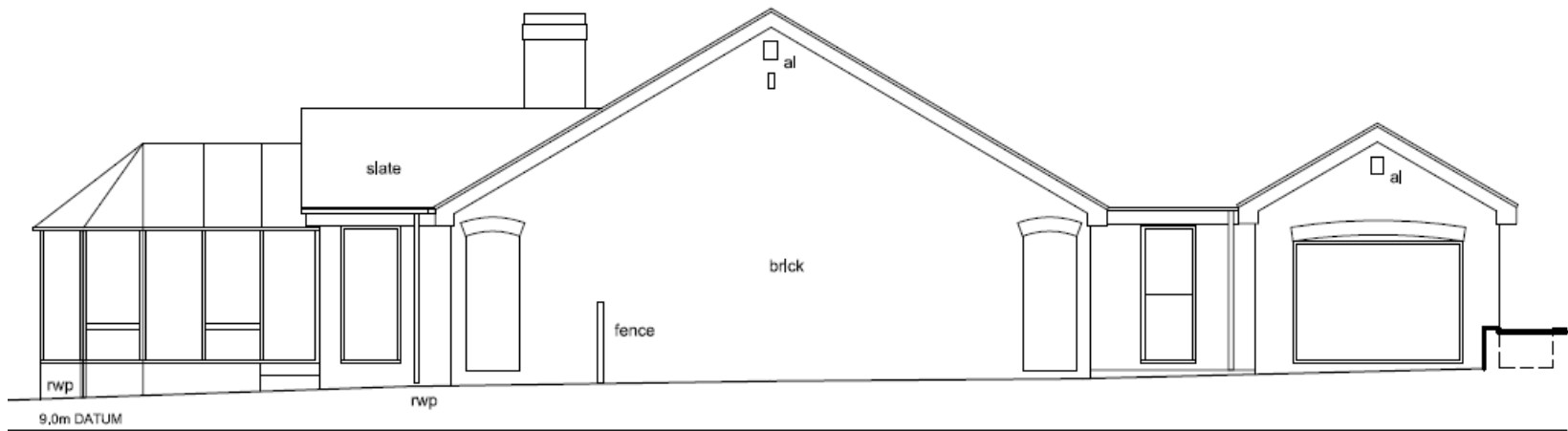
EAST ELEVATION
