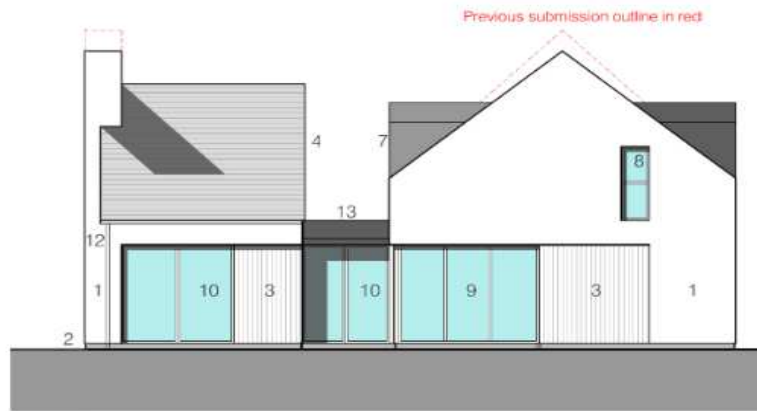
South Elevation
