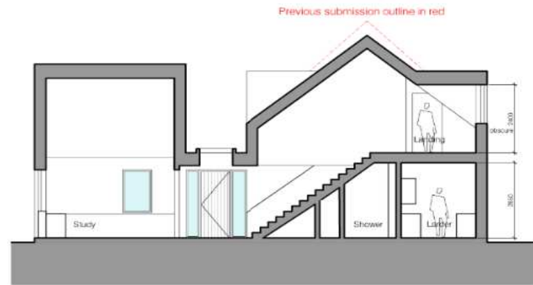
Cross Section
