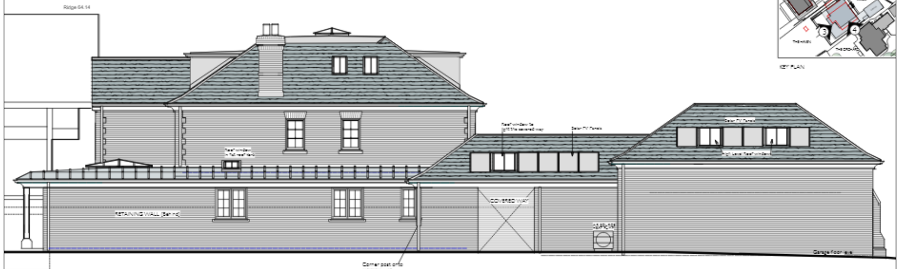
3. SOUTH WEST ELEVATION
