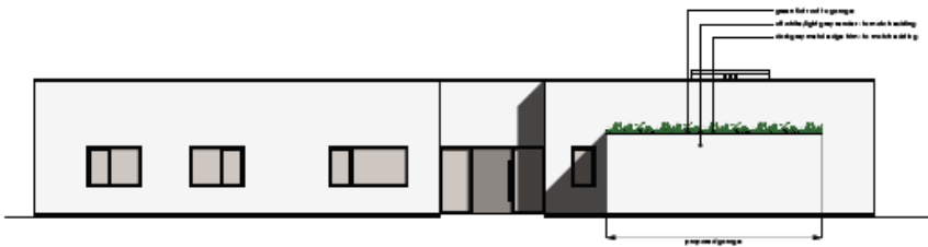
west (front) elevation (not) elevation
