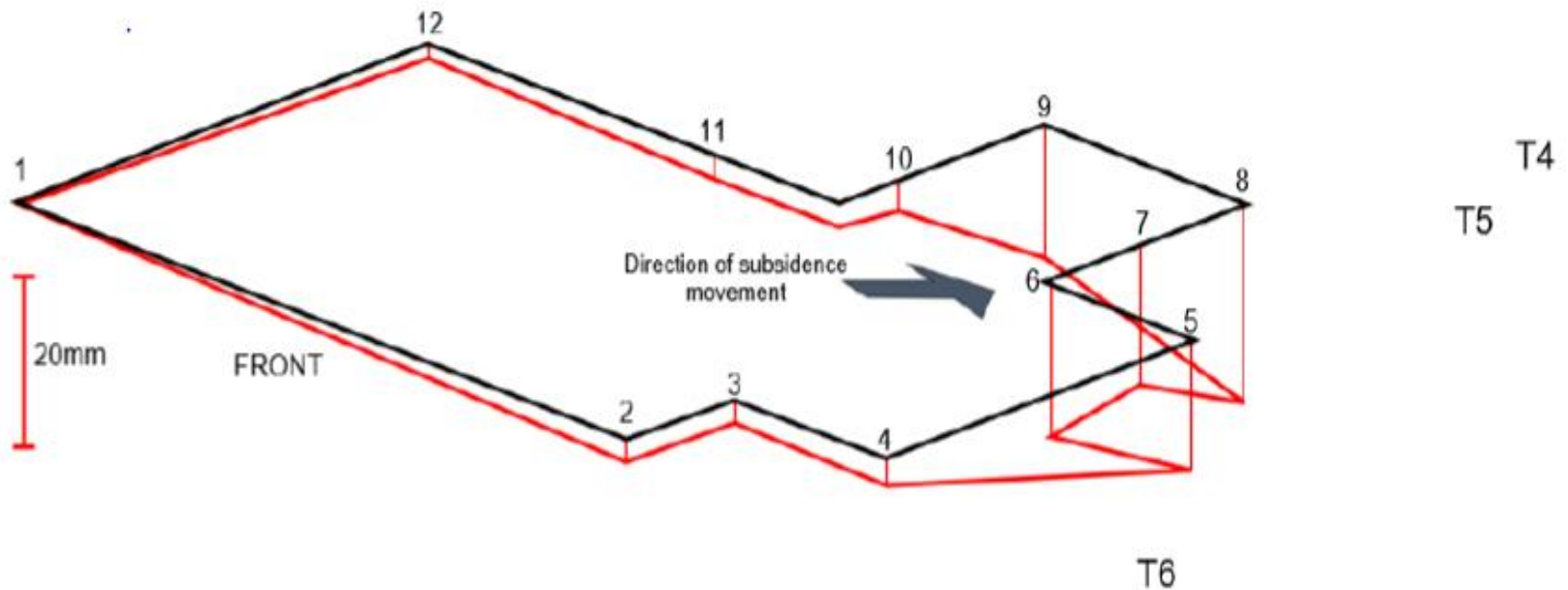
Figure 4. Isometric sketch showing the amplitude of movements at each monitoring location. The focus of movement is at markers 5 - 9 at the rear right hand corner, closest to oak T5.
