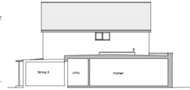
Side Elevation / Section (West)
